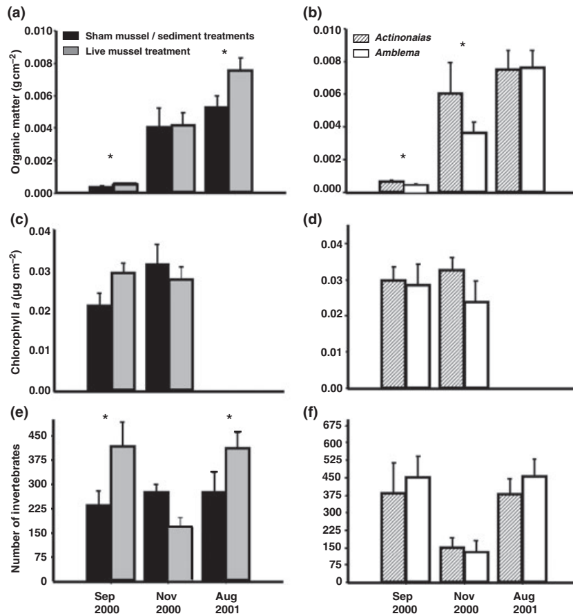
Fig. 2 Mean ± 1 SE for sediment response variables. (a), (c) and (e) are ANOVA comparisons of live mussel versus sham mussel/sediment treatments. (b), (d) and (f) are ANCOVA comparisons of the two species. Asterisks represent significant differences from multiple comparison procedures.
